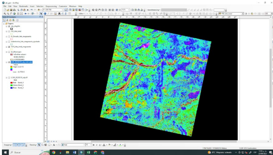
Figure 30. NDVI results
